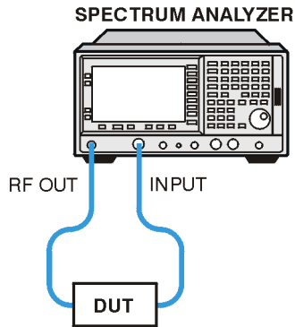
Figure 2-1 Transmission Measurement Test Setup
