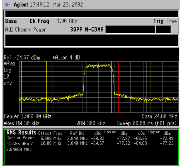
Figure 2-32 ACP Measurement on a Base Station W-CDMA Signal
