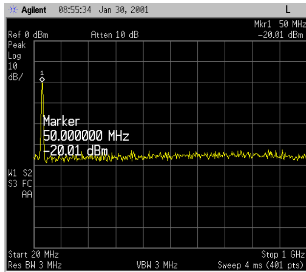
Figure 1-14 Detected Signal
