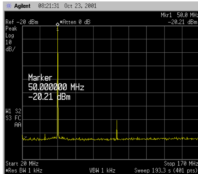
Figure 2-23 Longer Sweep Times are Required Without Segmented Sweep
