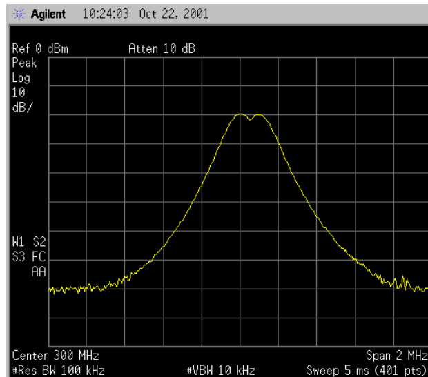
Figure 1-7 Resolving Signals of Equal Amplitude After Reducing the Video Bandwidth
