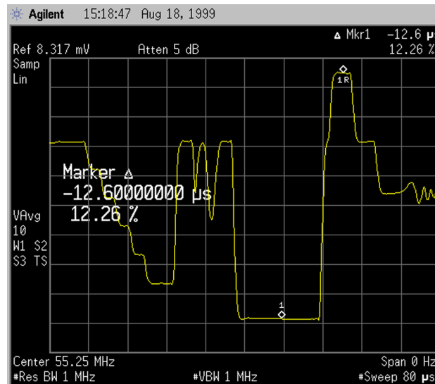
Figure 2-41 Measuring Marker Delta (%) for Depth of Modulation (NTSC)
