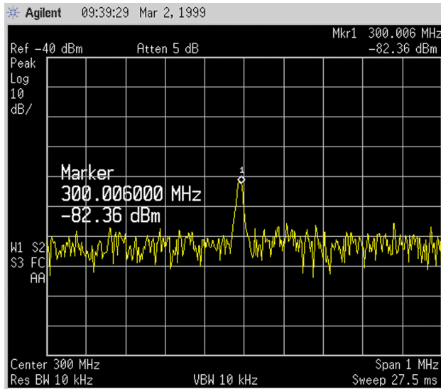
Figure 1-26 Low-Level Signal
